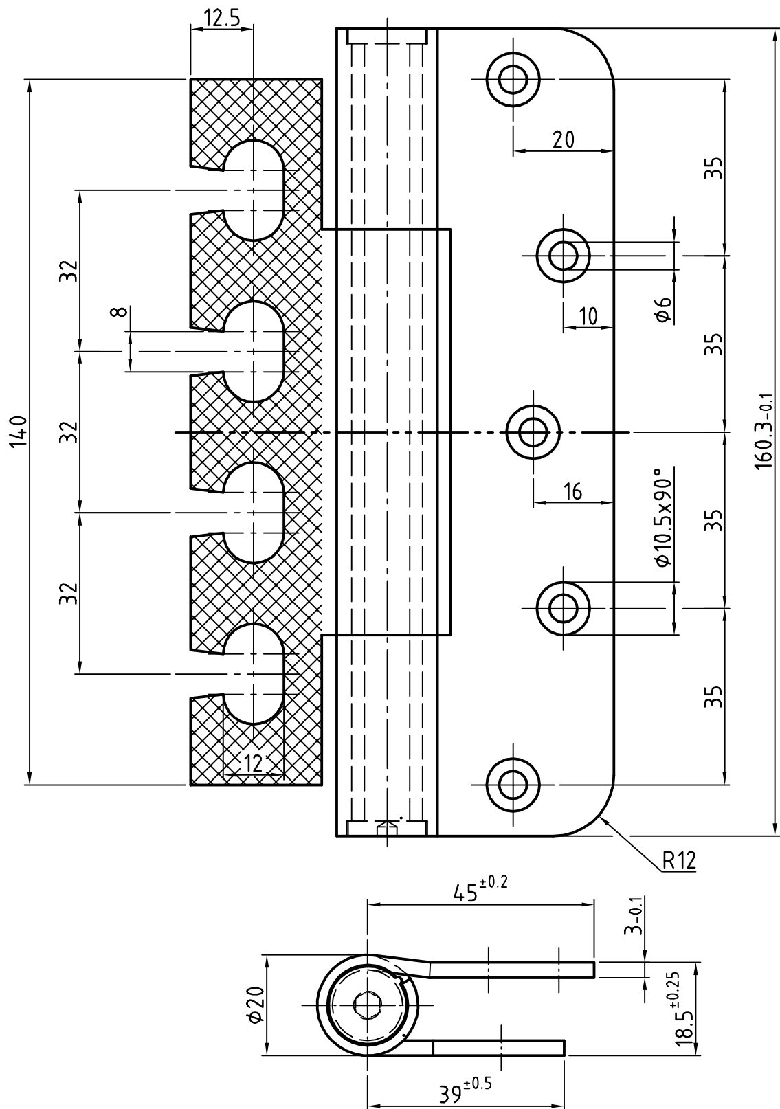
3D Projectscharnier 060-3/160
